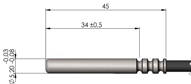
Temperature sensor
